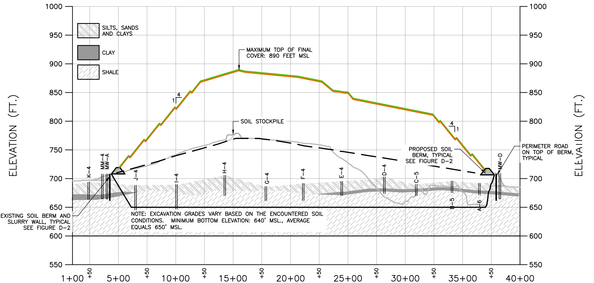
ALIGNMENT A SECTION SCALE H:1"=500'; V:1"=100'
